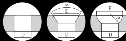
No Chamfer Conical Chamfer Spherical Chamfer
